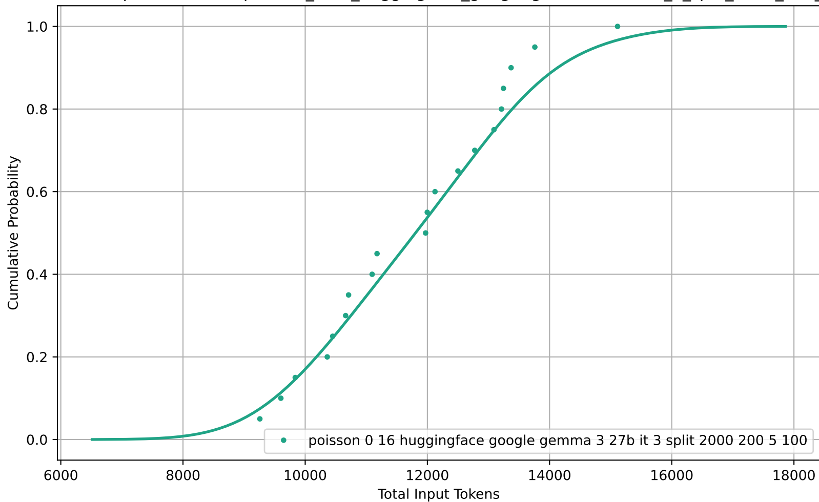
CDF of Total Input Tokens for poisson_0-16_huggingface_google-gemma-3-27b-it_3_split_2000_200_5_100
