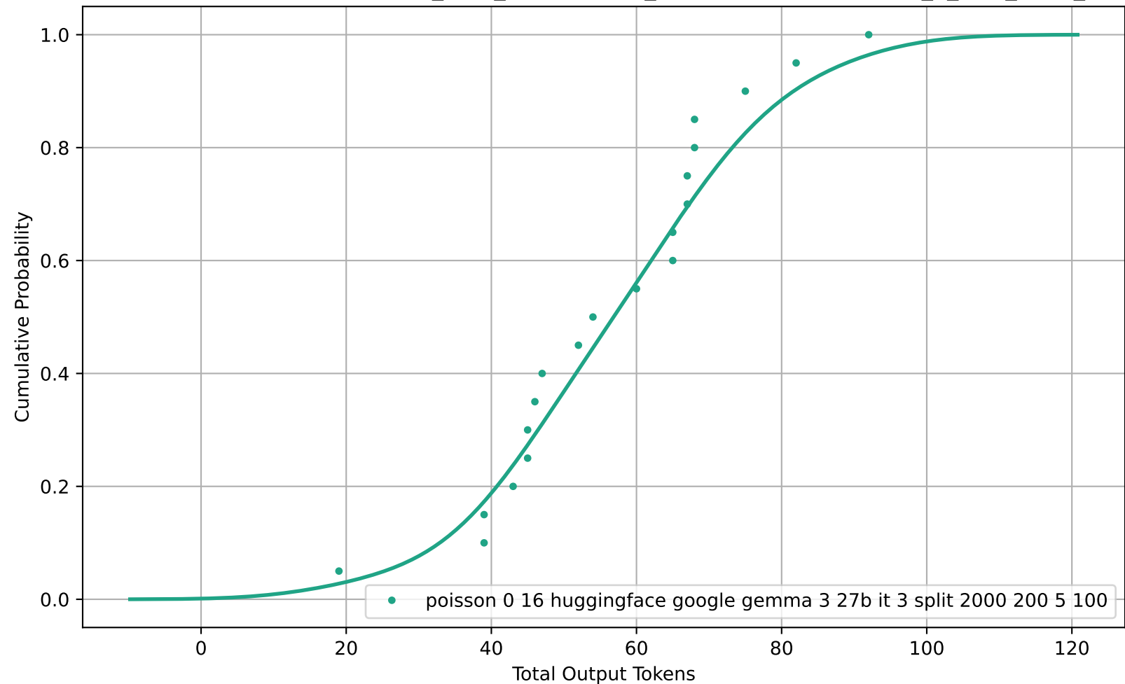
CDF of Total Output Tokens for poisson_0-16_huggingface_google-gemma-3-27b-it_3_split_2000_200_5_100
