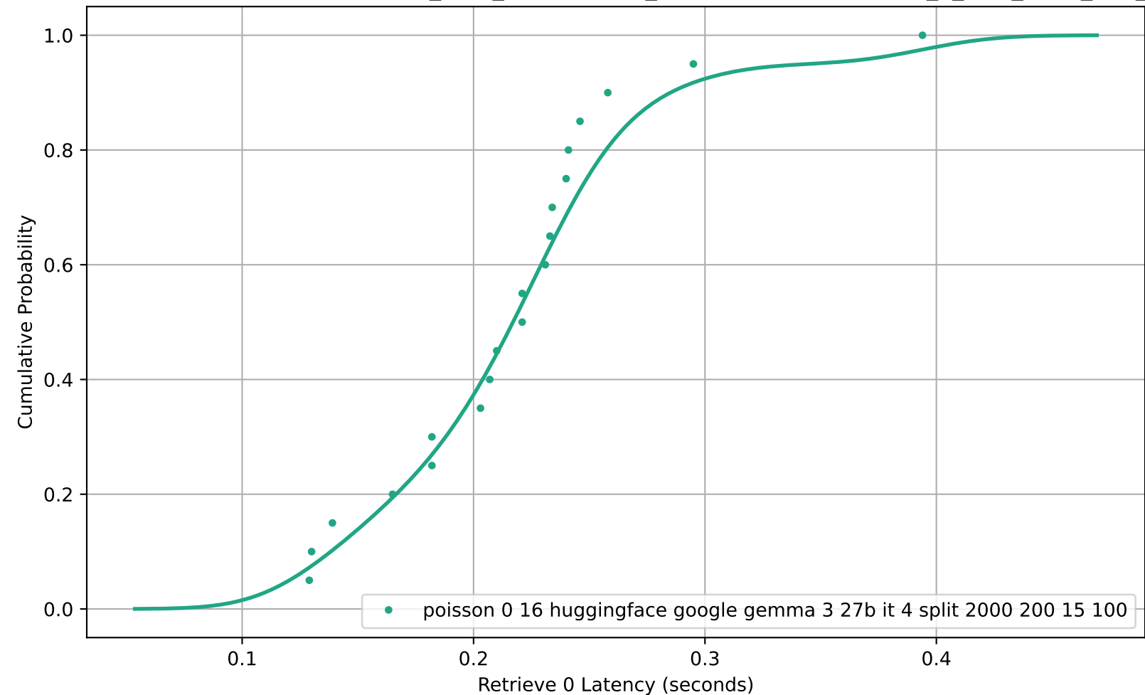
CDF of Retrieve 0 Latency for poisson_0-16_huggingface_google-gemma-3-27b-it_4_split_2000_200_15_100
