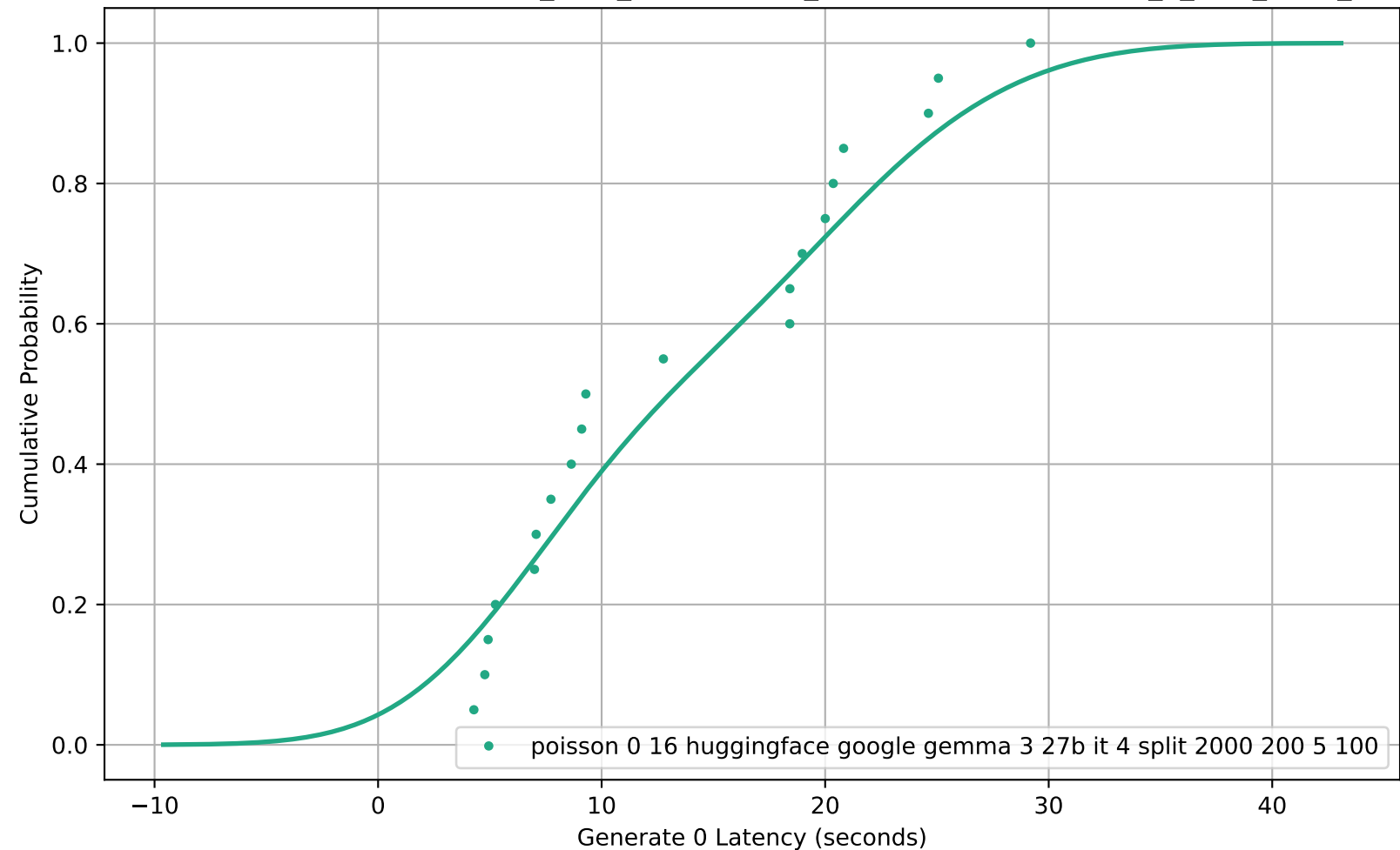
CDF of Generate 0 Latency for poisson_0-16_huggingface_google-gemma-3-27b-it_4_split_2000_200_5_100
