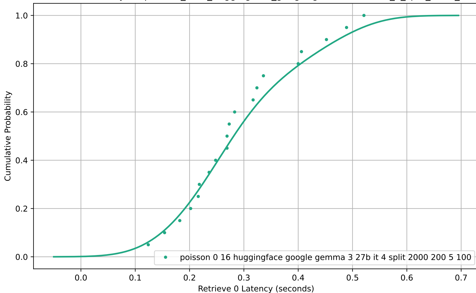
CDF of Retrieve 0 Latency for poisson_0-16_huggingface_google-gemma-3-27b-it_4_split_2000_200_5_100
