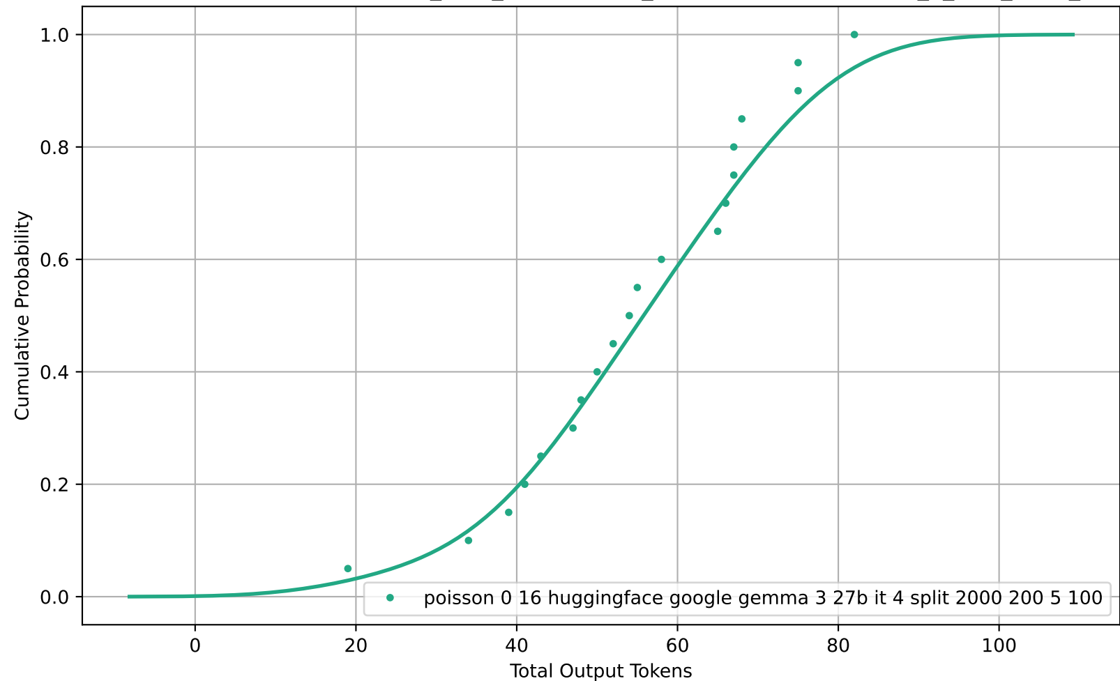
CDF of Total Output Tokens for poisson_0-16_huggingface_google-gemma-3-27b-it_4_split_2000_200_5_100
