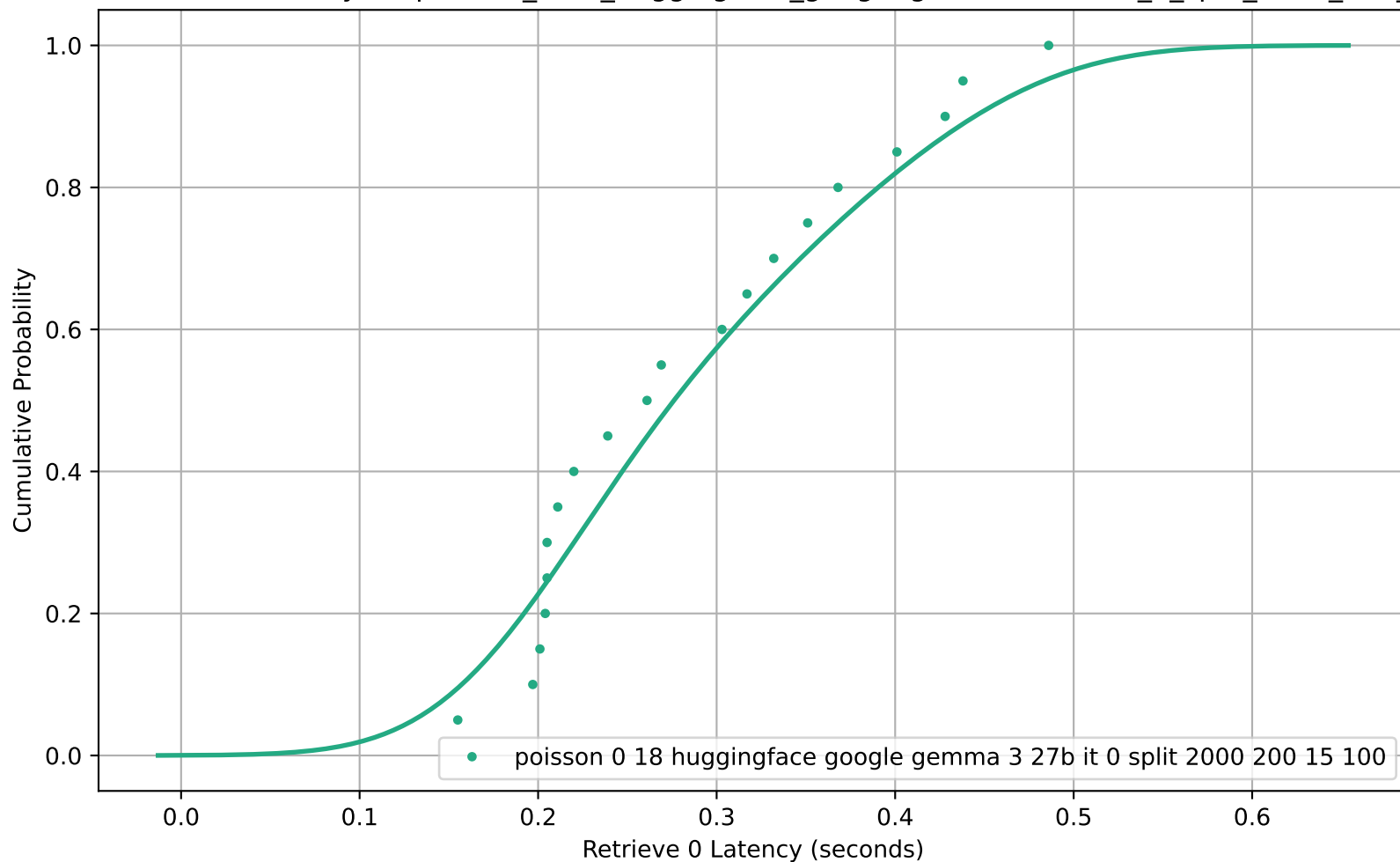
CDF of Retrieve 0 Latency for poisson_0-18_huggingface_google-gemma-3-27b-it_0_split_2000_200_15_100
