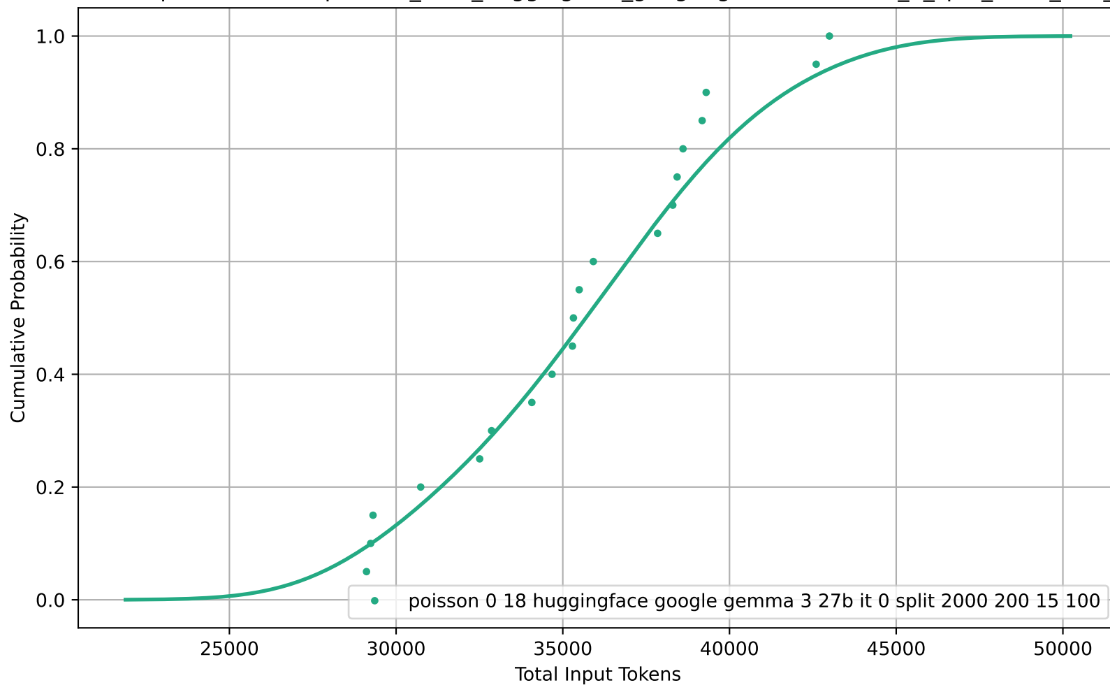
CDF of Total Input Tokens for poisson_0-18_huggingface_google-gemma-3-27b-it_0_split_2000_200_15_100
