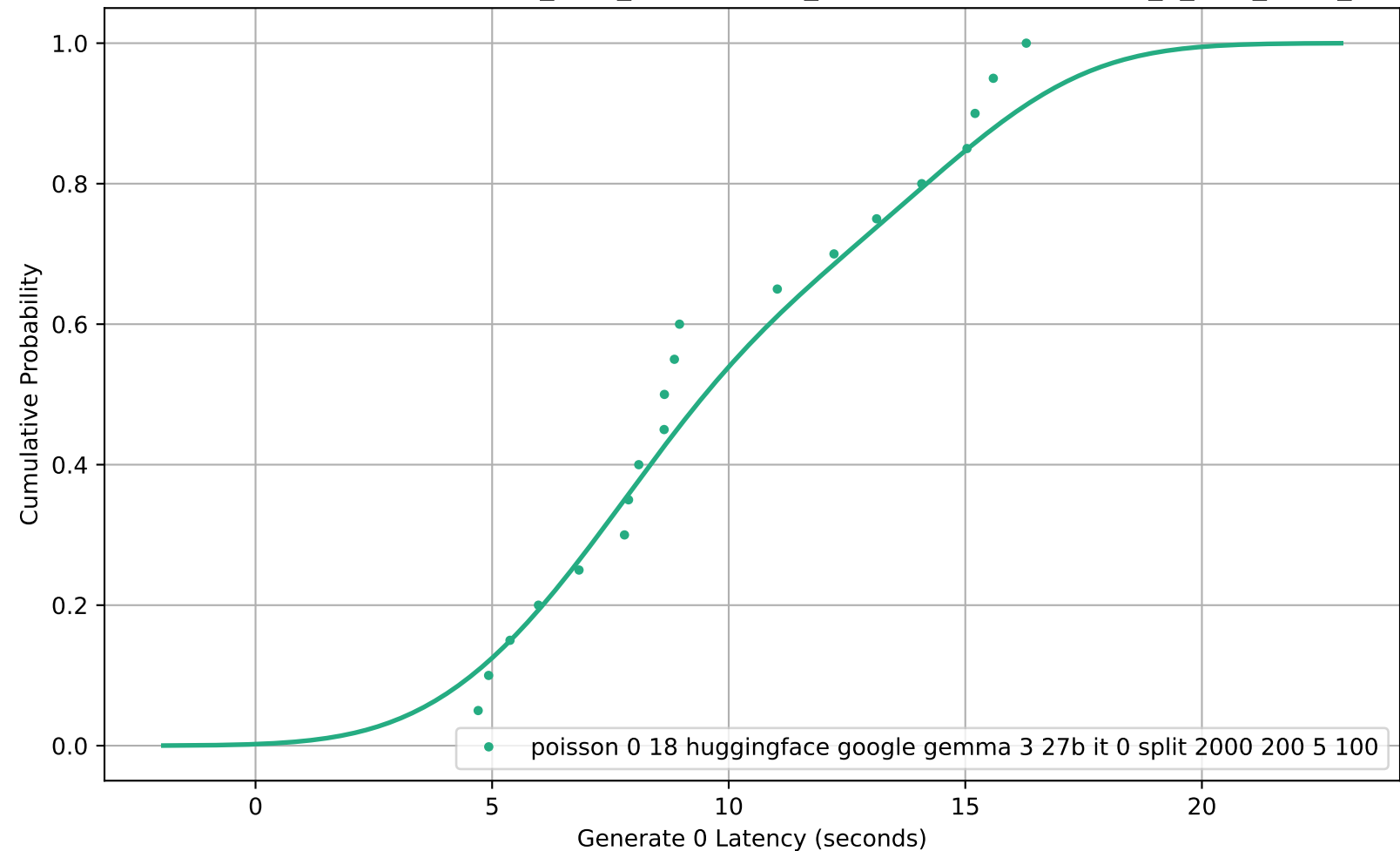
CDF of Generate 0 Latency for poisson_0-18_huggingface_google-gemma-3-27b-it_0_split_2000_200_5_100
