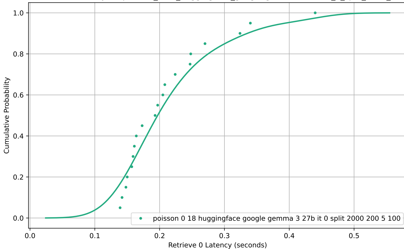
CDF of Retrieve 0 Latency for poisson_0-18_huggingface_google-gemma-3-27b-it_0_split_2000_200_5_100
