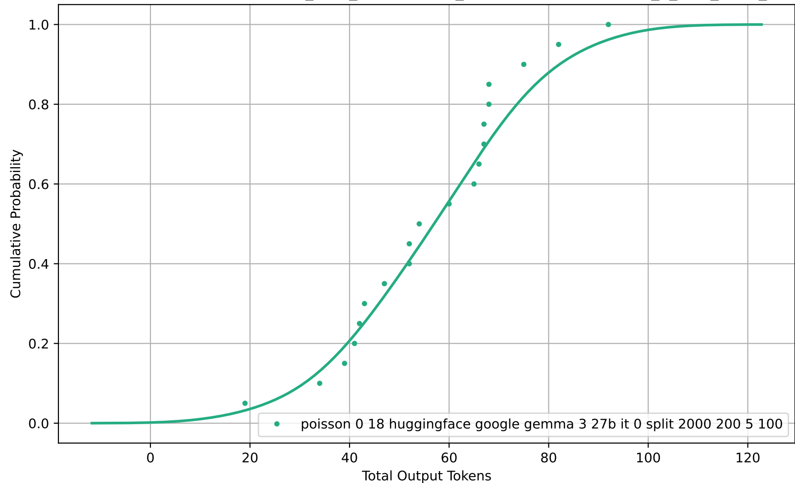
CDF of Total Output Tokens for poisson_0-18_huggingface_google-gemma-3-27b-it_0_split_2000_200_5_100
