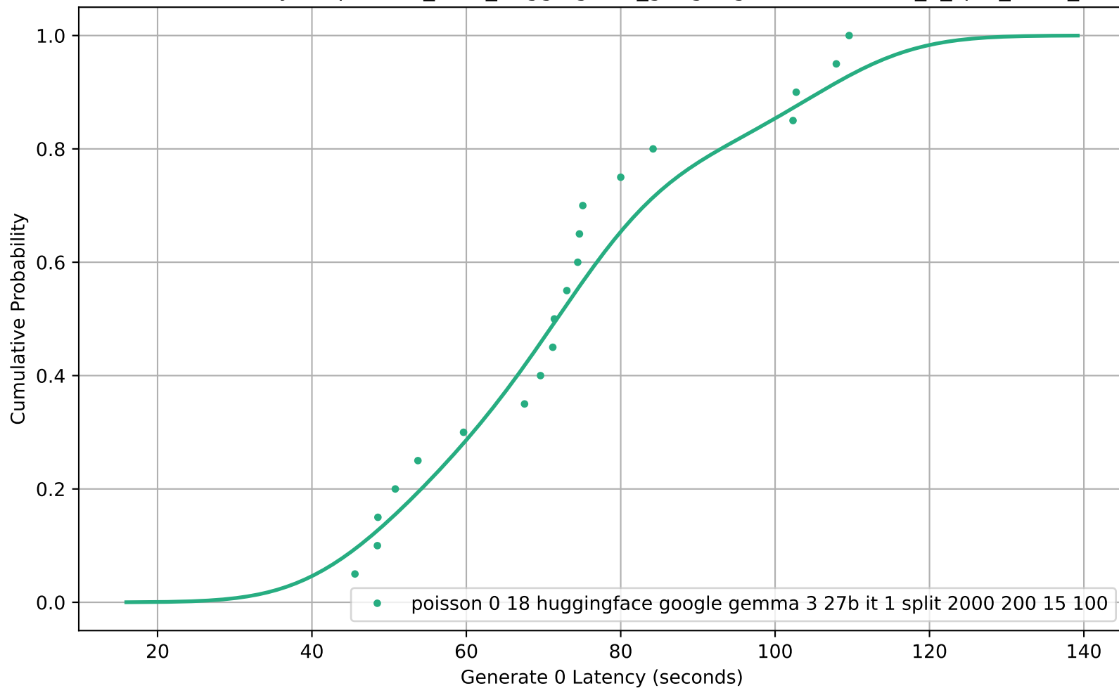
CDF of Generate 0 Latency for poisson_0-18_huggingface_google-gemma-3-27b-it_1_split_2000_200_15_100
