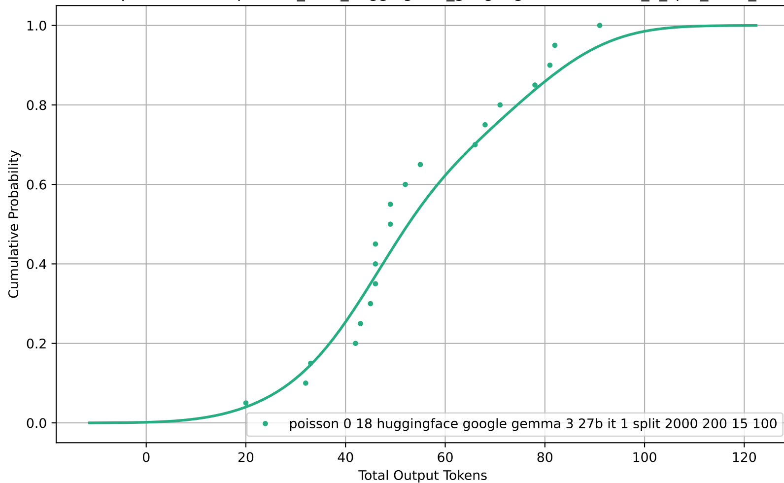
CDF of Total Output Tokens for poisson_0-18_huggingface_google-gemma-3-27b-it_1_split_2000_200_15_100
