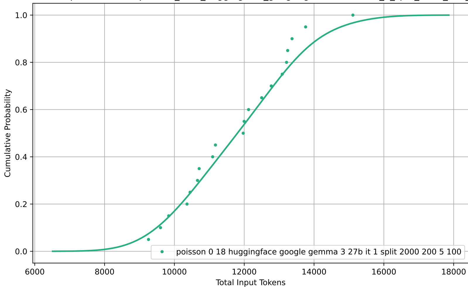
CDF of Total Input Tokens for poisson_0-18_huggingface_google-gemma-3-27b-it_1_split_2000_200_5_100
