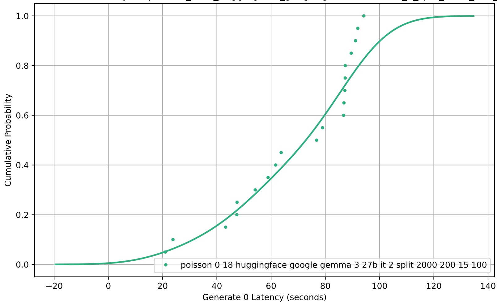
CDF of Generate 0 Latency for poisson_0-18_huggingface_google-gemma-3-27b-it_2_split_2000_200_15_100
