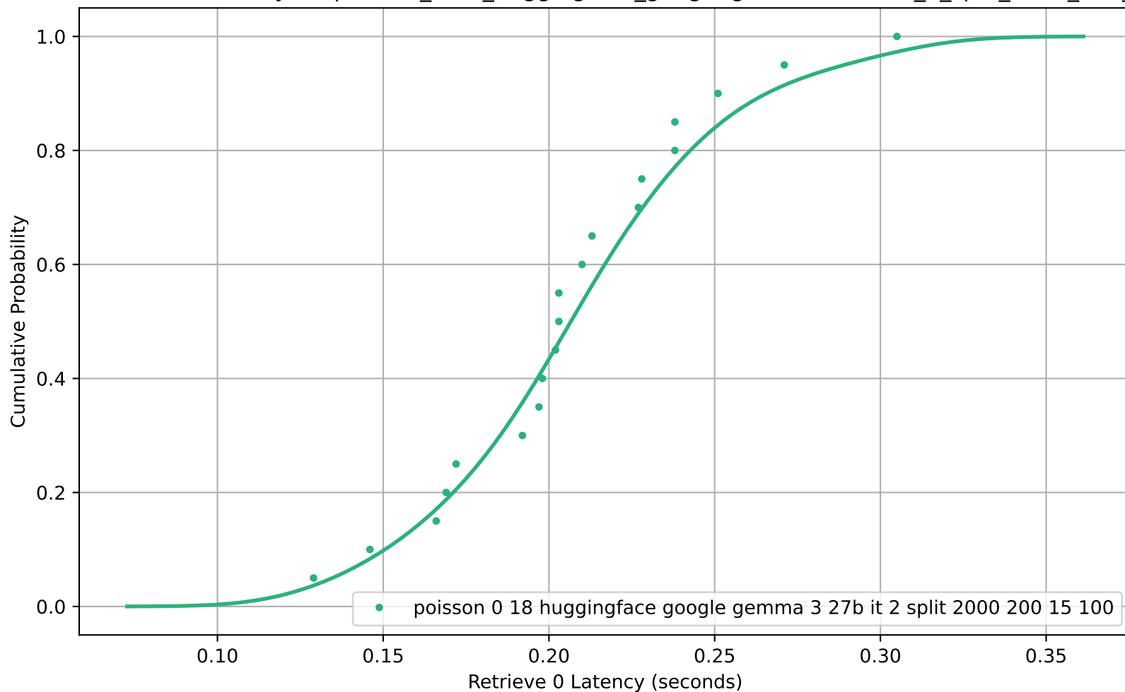
CDF of Retrieve 0 Latency for poisson_0-18_huggingface_google-gemma-3-27b-it_2_split_2000_200_15_100
