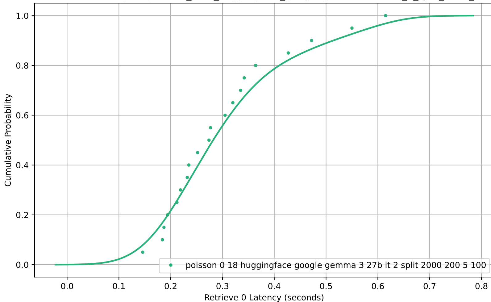
CDF of Retrieve 0 Latency for poisson_0-18_huggingface_google-gemma-3-27b-it_2_split_2000_200_5_100
