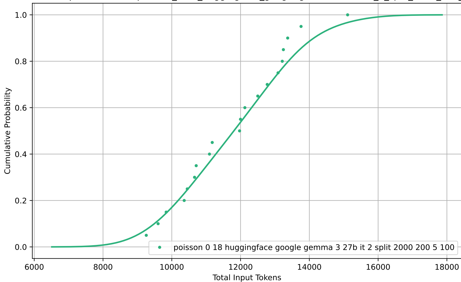
CDF of Total Input Tokens for poisson_0-18_huggingface_google-gemma-3-27b-it_2_split_2000_200_5_100
