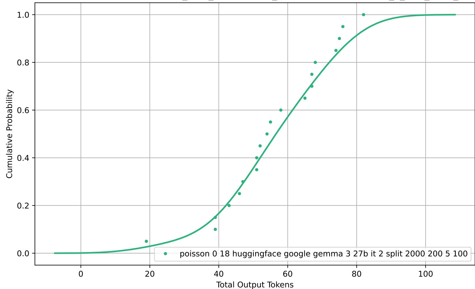
CDF of Total Output Tokens for poisson_0-18_huggingface_google-gemma-3-27b-it_2_split_2000_200_5_100
