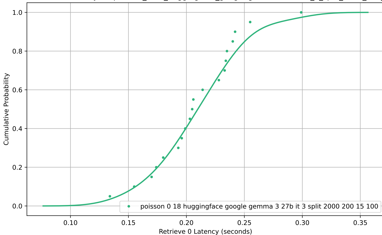
CDF of Retrieve 0 Latency for poisson_0-18_huggingface_google-gemma-3-27b-it_3_split_2000_200_15_100
