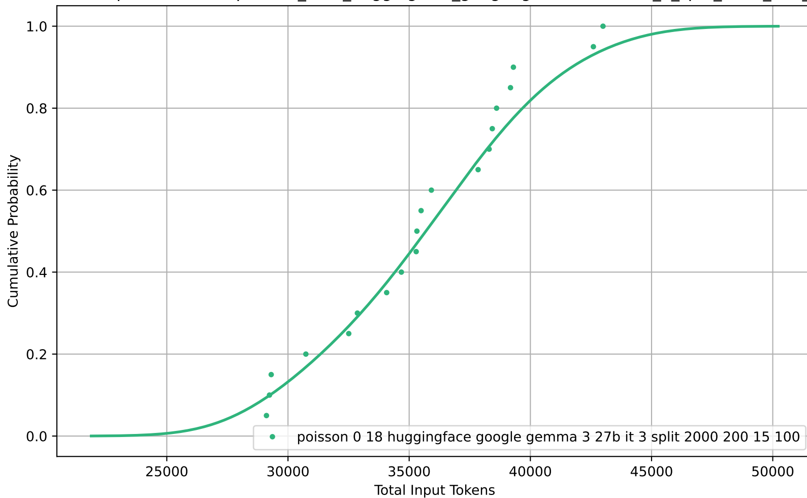
CDF of Total Input Tokens for poisson_0-18_huggingface_google-gemma-3-27b-it_3_split_2000_200_15_100
