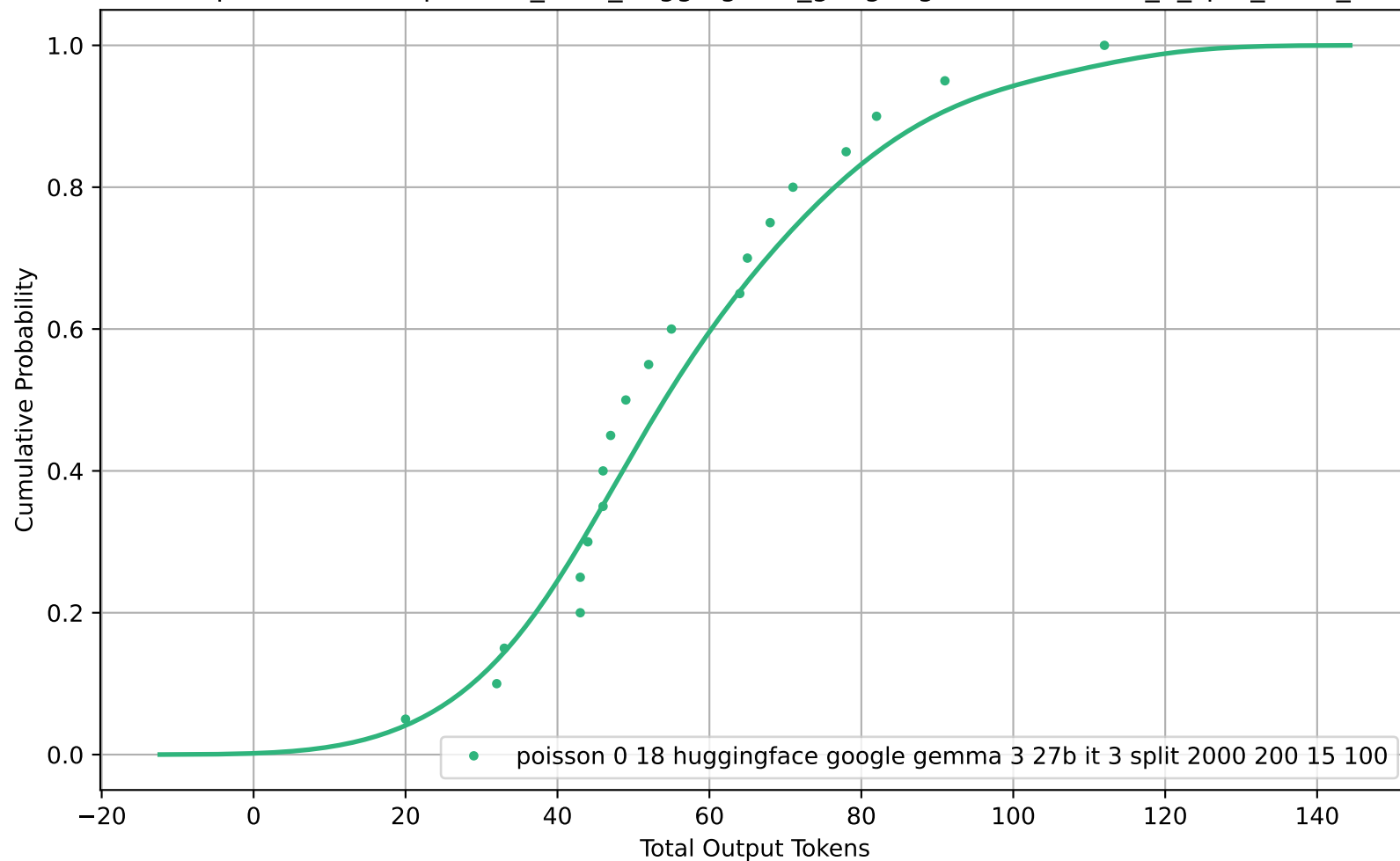
CDF of Total Output Tokens for poisson_0-18_huggingface_google-gemma-3-27b-it_3_split_2000_200_15_100
