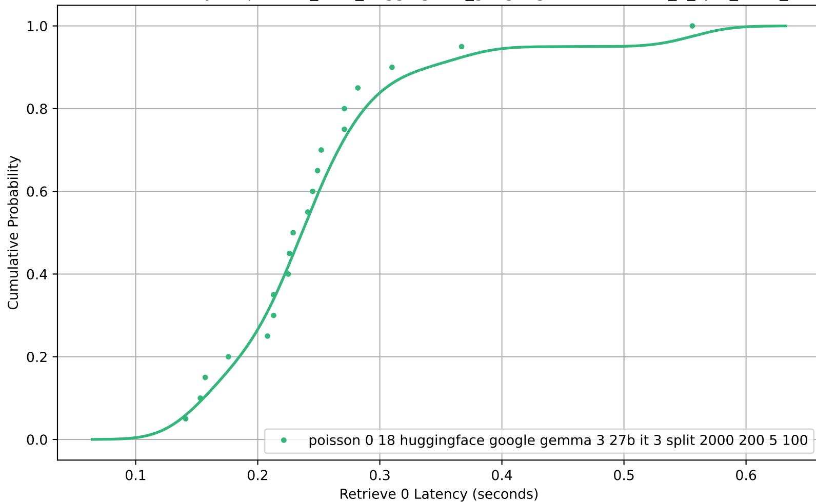
CDF of Retrieve 0 Latency for poisson_0-18_huggingface_google-gemma-3-27b-it_3_split_2000_200_5_100
