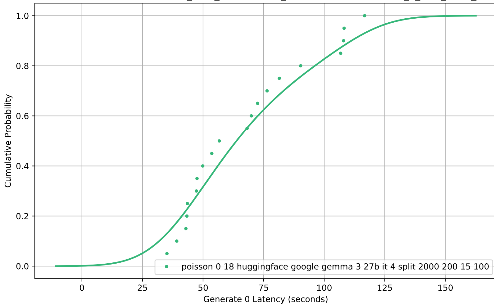
CDF of Generate 0 Latency for poisson_0-18_huggingface_google-gemma-3-27b-it_4_split_2000_200_15_100
