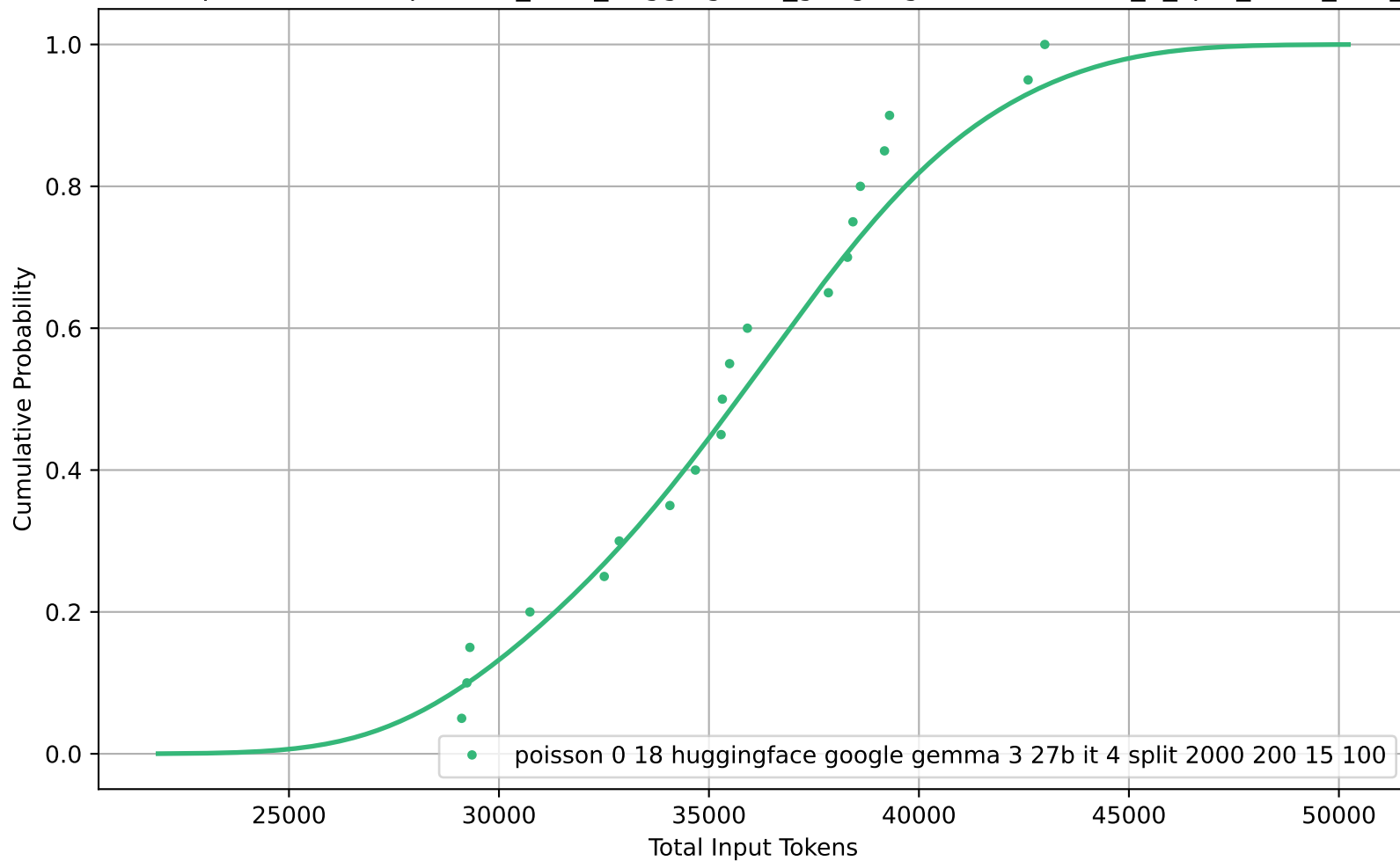
CDF of Total Input Tokens for poisson_0-18_huggingface_google-gemma-3-27b-it_4_split_2000_200_15_100
