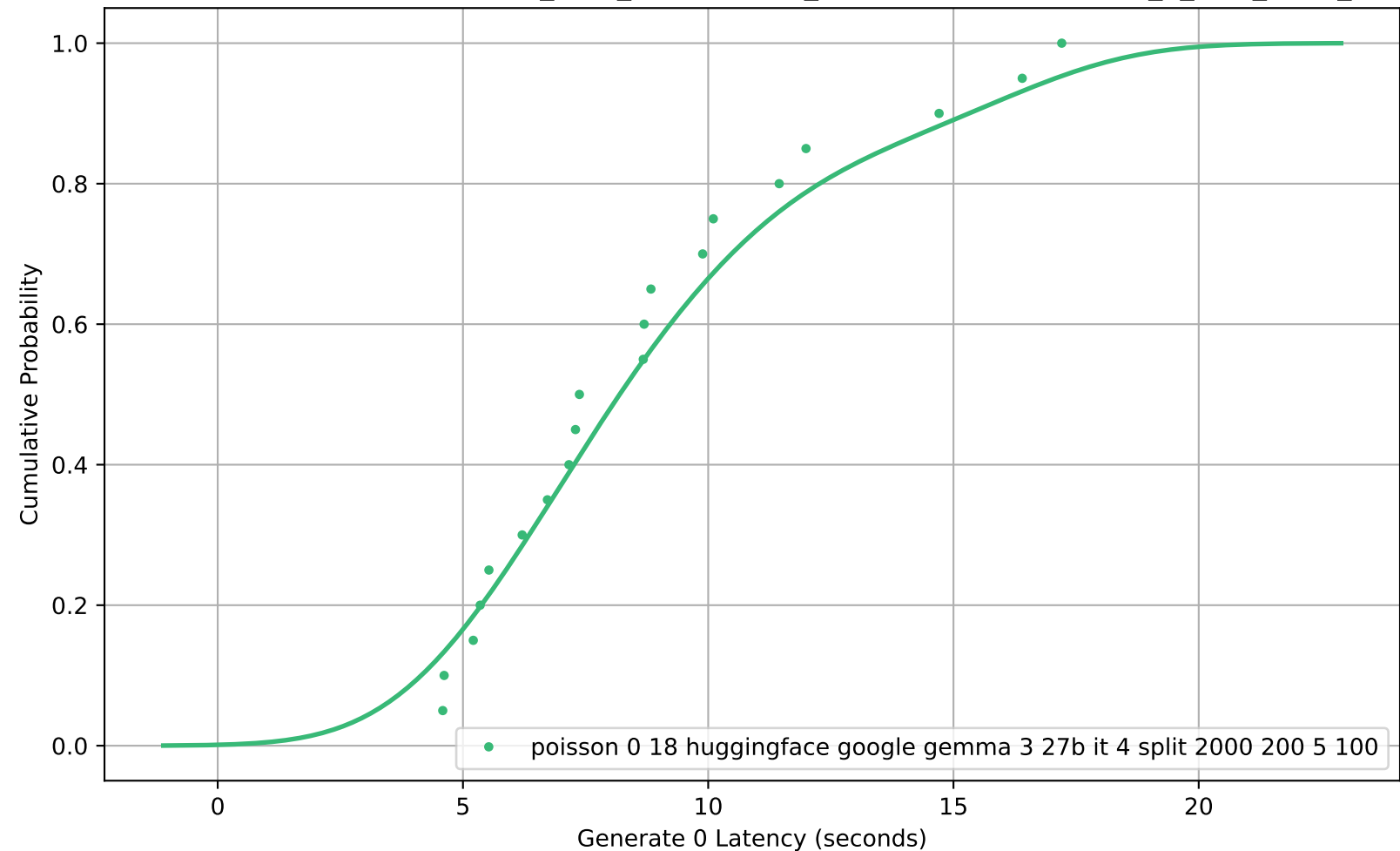
CDF of Generate 0 Latency for poisson_0-18_huggingface_google-gemma-3-27b-it_4_split_2000_200_5_100
