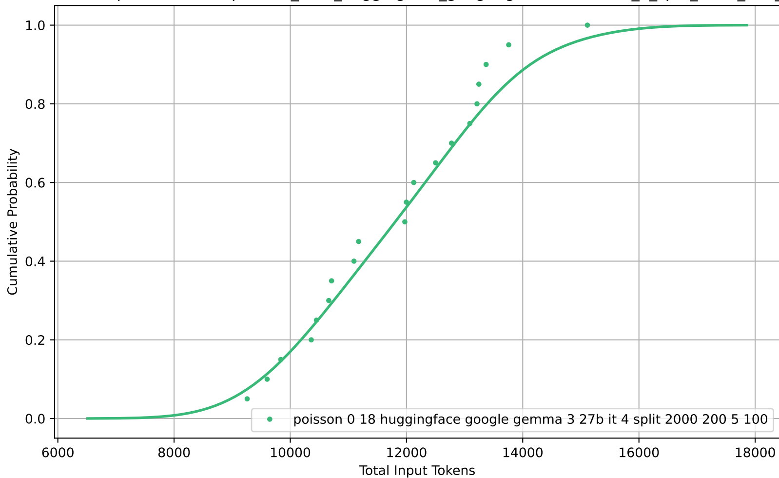
CDF of Total Input Tokens for poisson_0-18_huggingface_google-gemma-3-27b-it_4_split_2000_200_5_100
