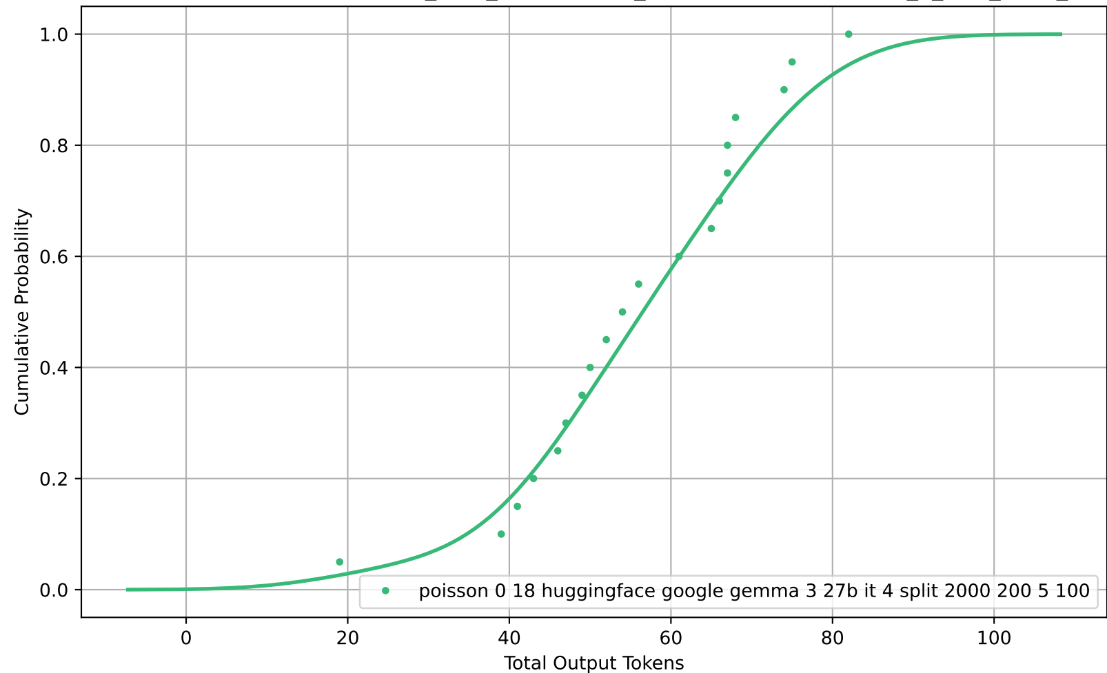
CDF of Total Output Tokens for poisson_0-18_huggingface_google-gemma-3-27b-it_4_split_2000_200_5_100
