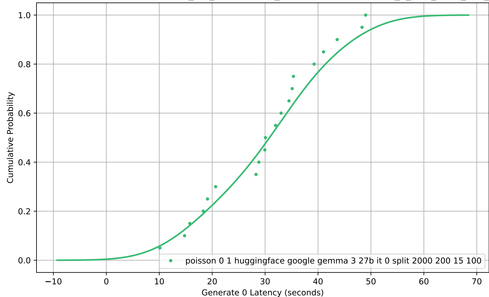
CDF of Generate 0 Latency for poisson_0-1_huggingface_google-gemma-3-27b-it_0_split_2000_200_15_100
