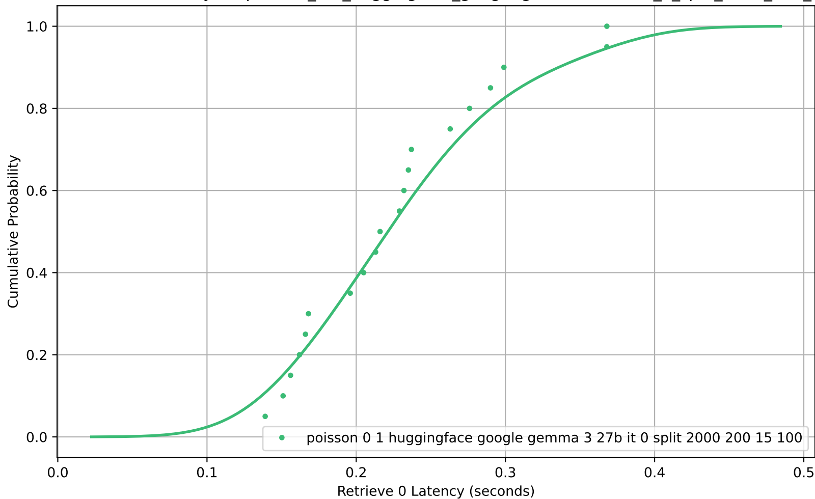
CDF of Retrieve 0 Latency for poisson_0-1_huggingface_google-gemma-3-27b-it_0_split_2000_200_15_100
