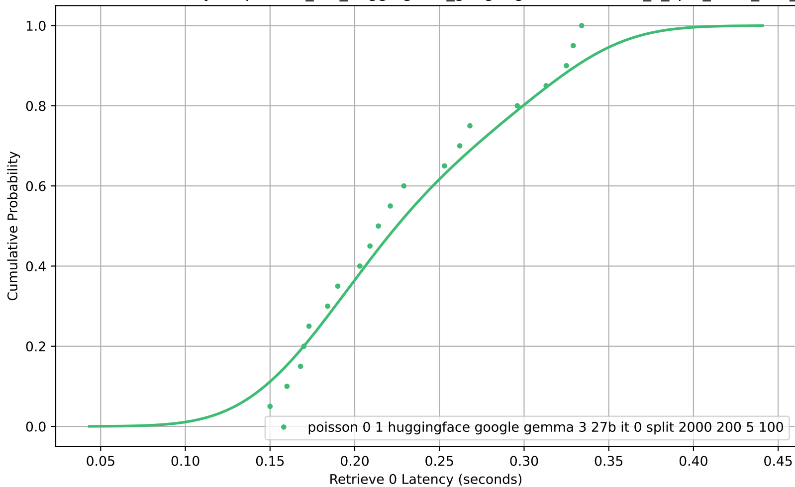
CDF of Retrieve 0 Latency for poisson_0-1_huggingface_google-gemma-3-27b-it_0_split_2000_200_5_100
