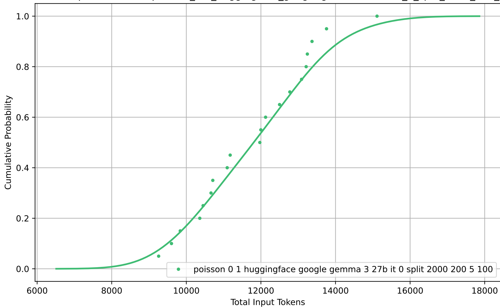
CDF of Total Input Tokens for poisson_0-1_huggingface_google-gemma-3-27b-it_0_split_2000_200_5_100
