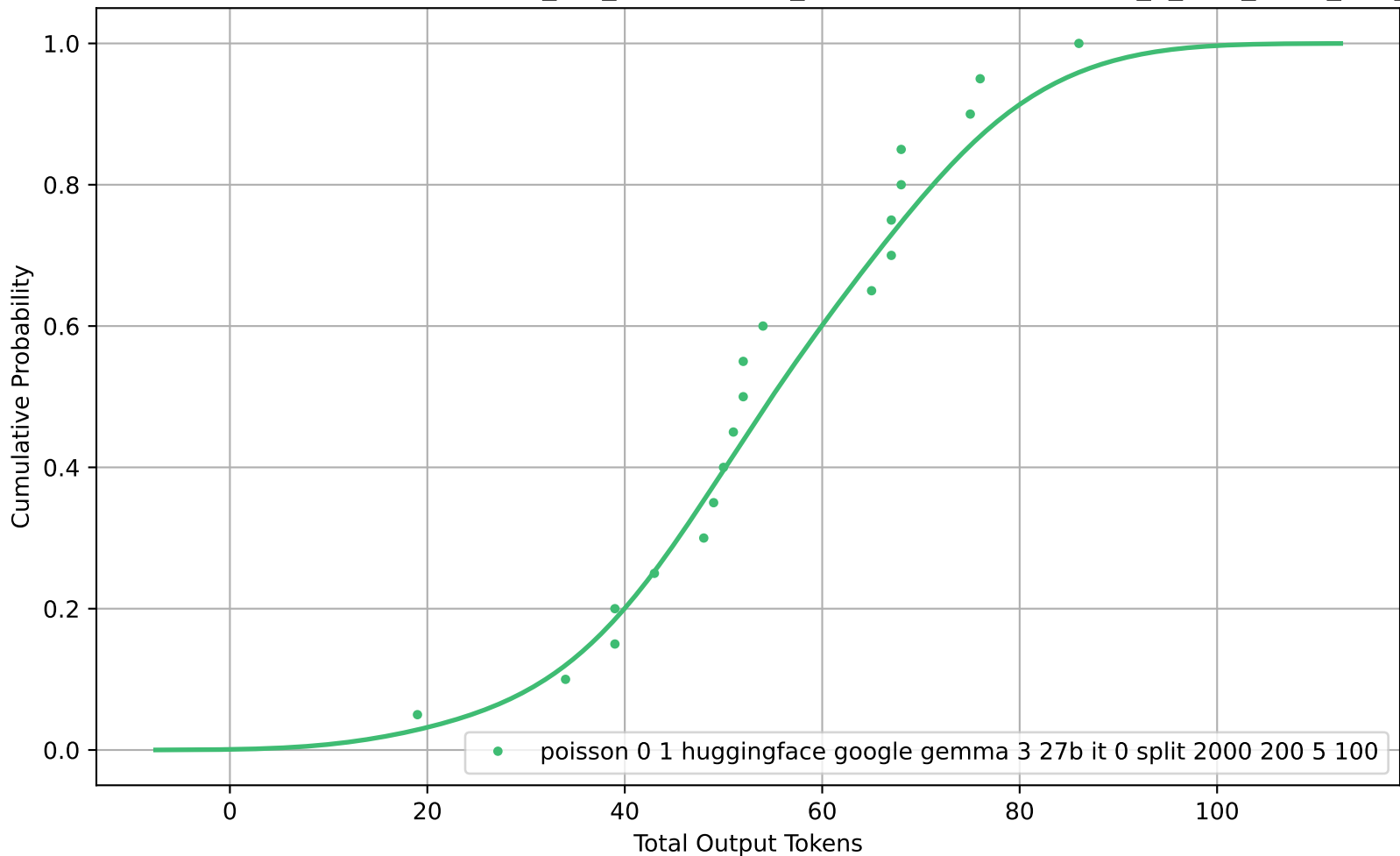
CDF of Total Output Tokens for poisson_0-1_huggingface_google-gemma-3-27b-it_0_split_2000_200_5_100
