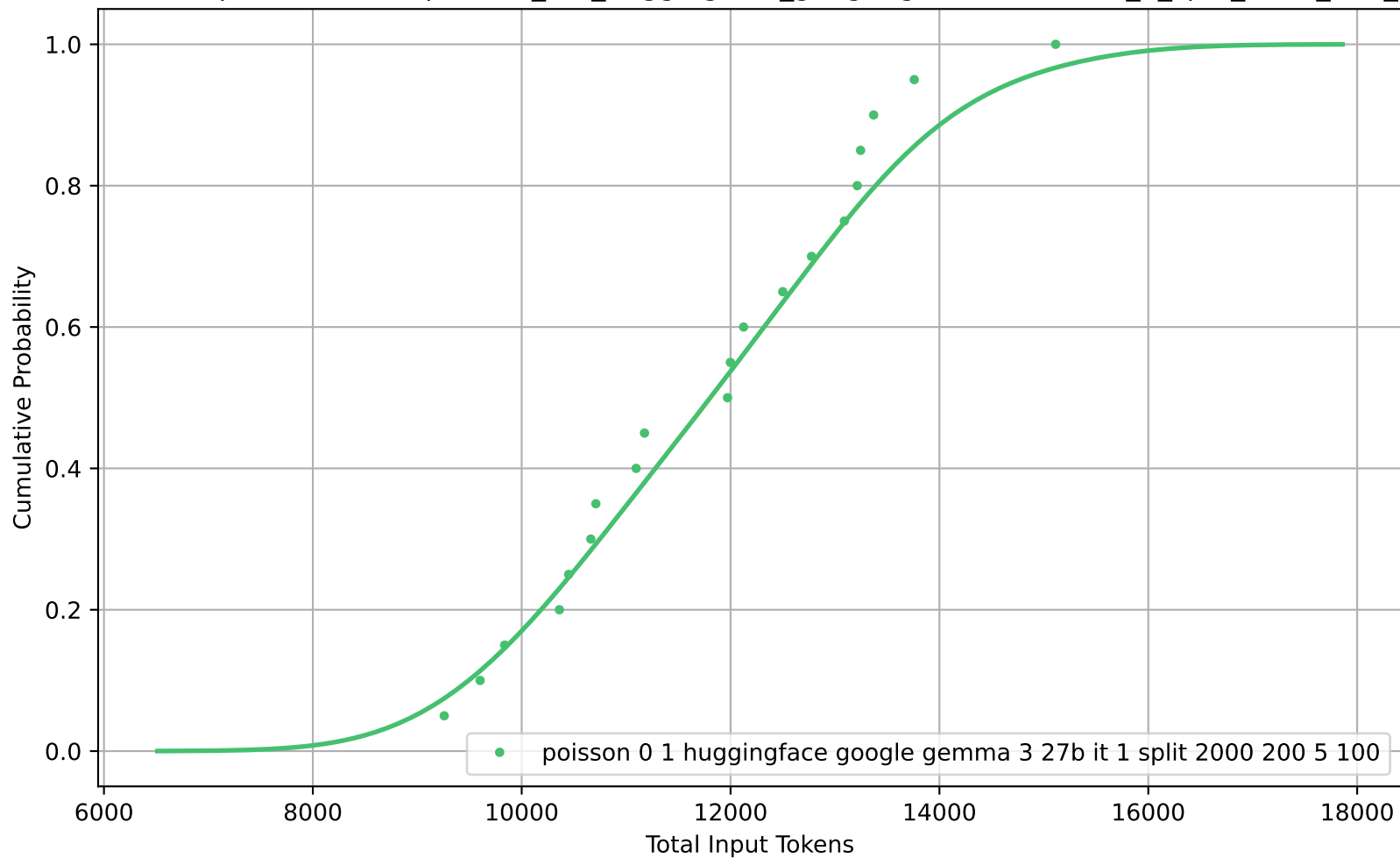
CDF of Total Input Tokens for poisson_0-1_huggingface_google-gemma-3-27b-it_1_split_2000_200_5_100
