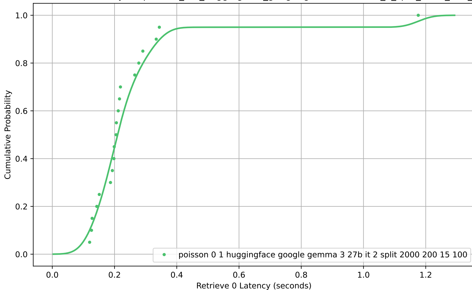
CDF of Retrieve 0 Latency for poisson_0-1_huggingface_google-gemma-3-27b-it_2_split_2000_200_15_100
