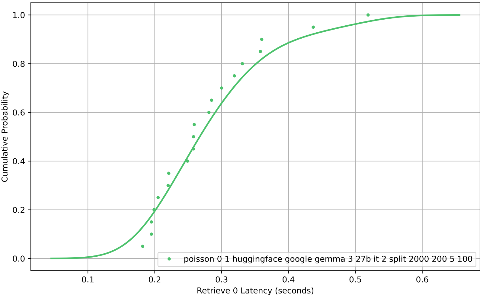
CDF of Retrieve 0 Latency for poisson_0-1_huggingface_google-gemma-3-27b-it_2_split_2000_200_5_100
