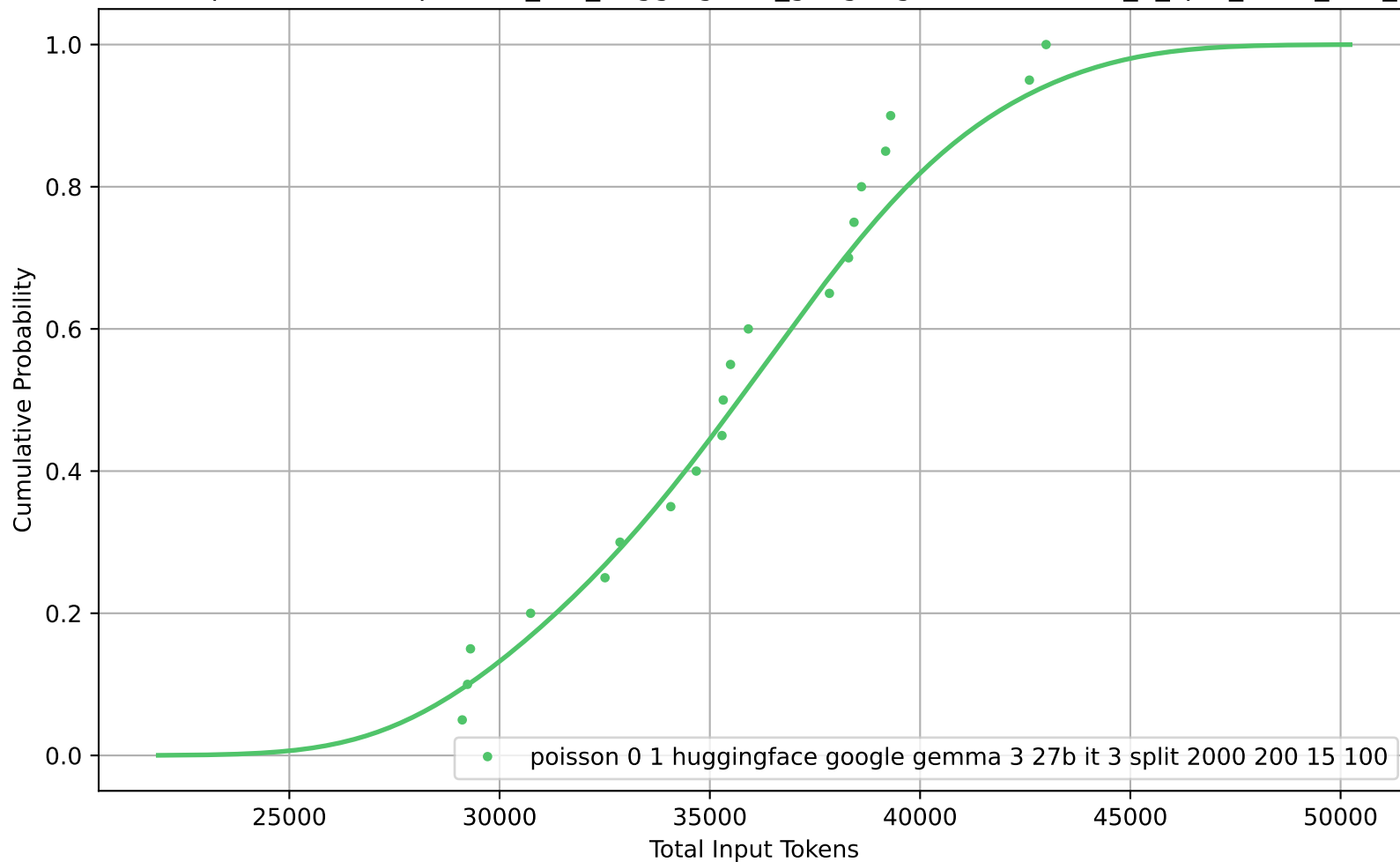
CDF of Total Input Tokens for poisson_0-1_huggingface_google-gemma-3-27b-it_3_split_2000_200_15_100
