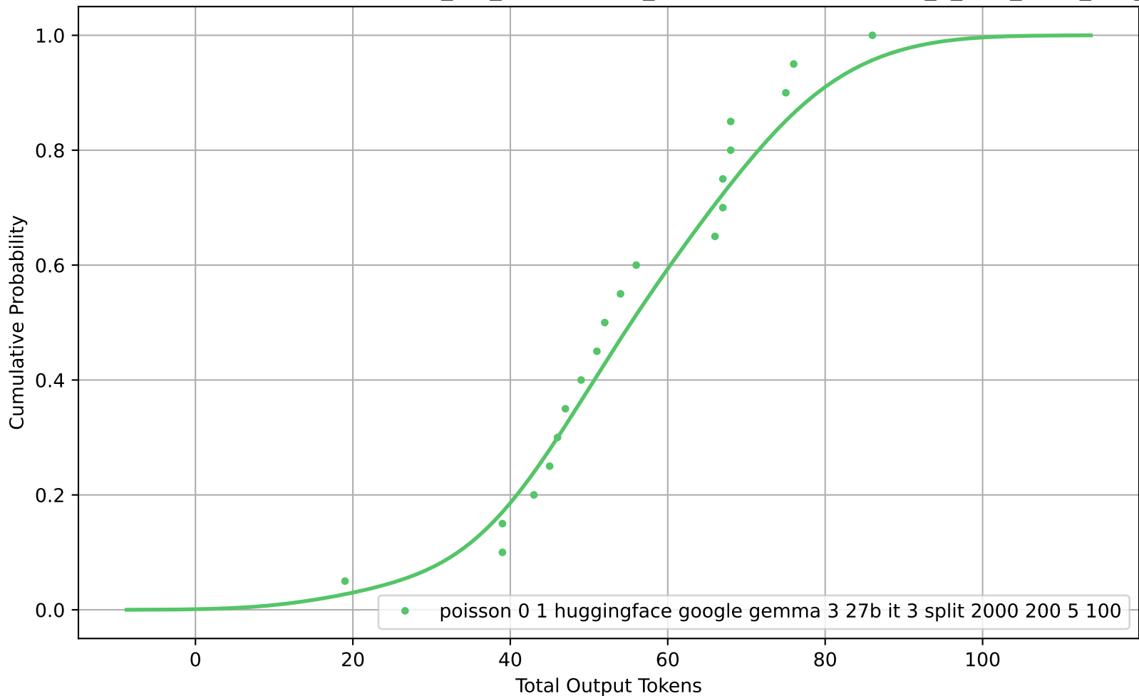
CDF of Total Output Tokens for poisson_0-1_huggingface_google-gemma-3-27b-it_3_split_2000_200_5_100
