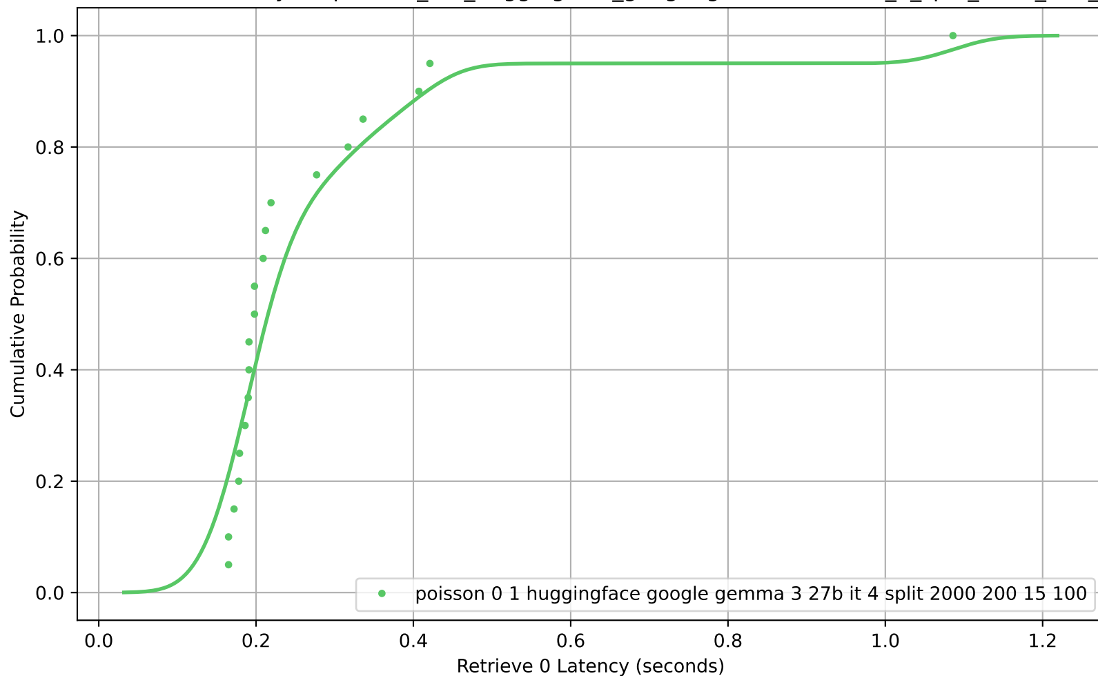
CDF of Retrieve 0 Latency for poisson_0-1_huggingface_google-gemma-3-27b-it_4_split_2000_200_15_100
