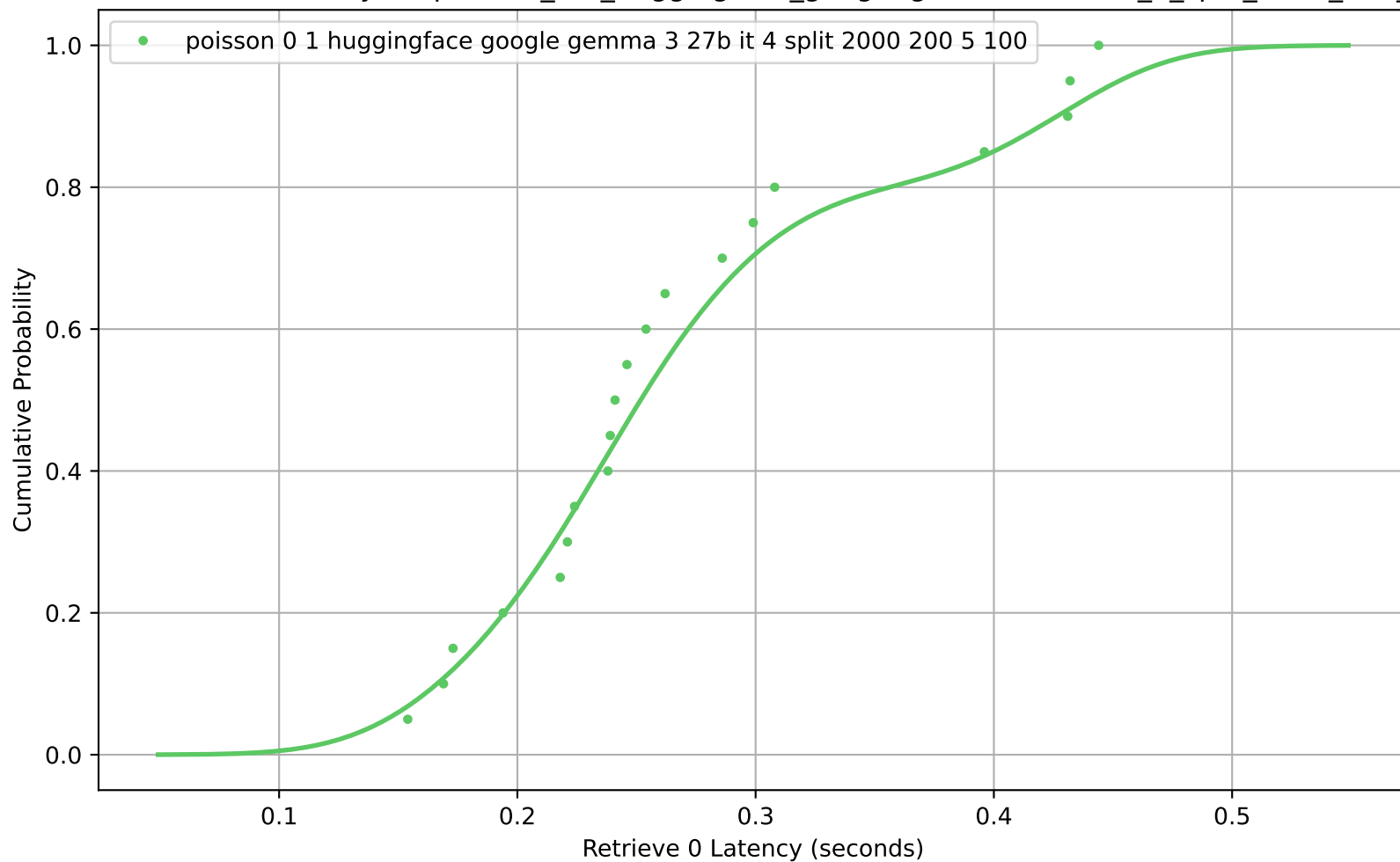
CDF of Retrieve 0 Latency for poisson_0-1_huggingface_google-gemma-3-27b-it_4_split_2000_200_5_100
