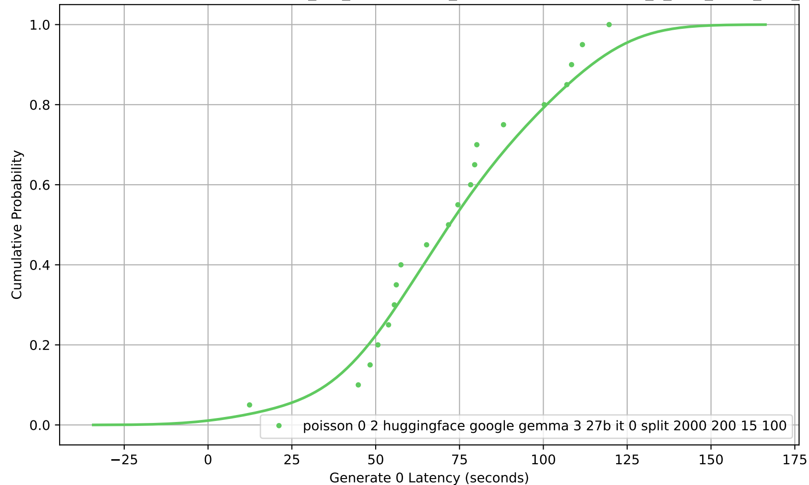
CDF of Generate 0 Latency for poisson_0-2_huggingface_google-gemma-3-27b-it_0_split_2000_200_15_100
