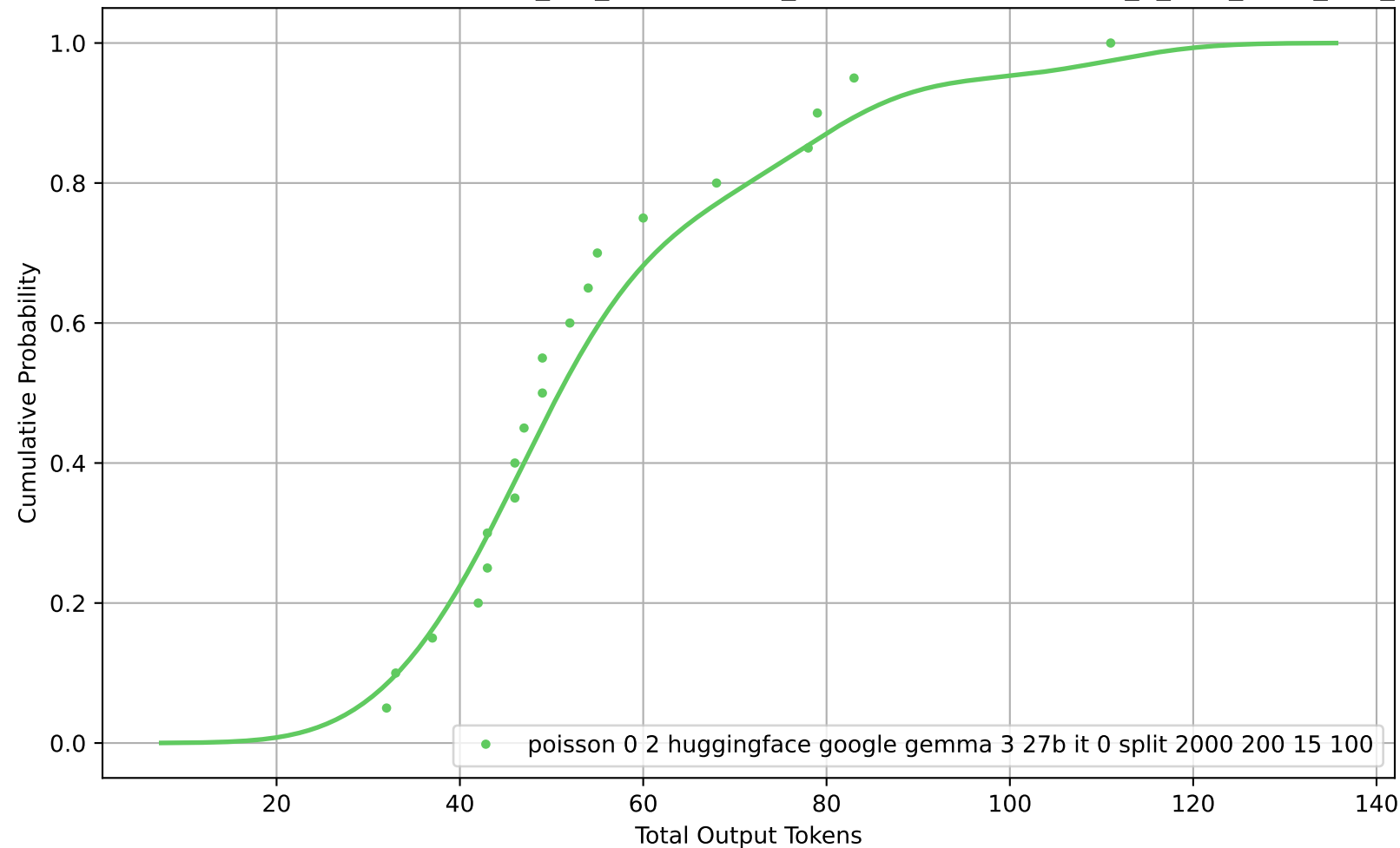
CDF of Total Output Tokens for poisson_0-2_huggingface_google-gemma-3-27b-it_0_split_2000_200_15_100
