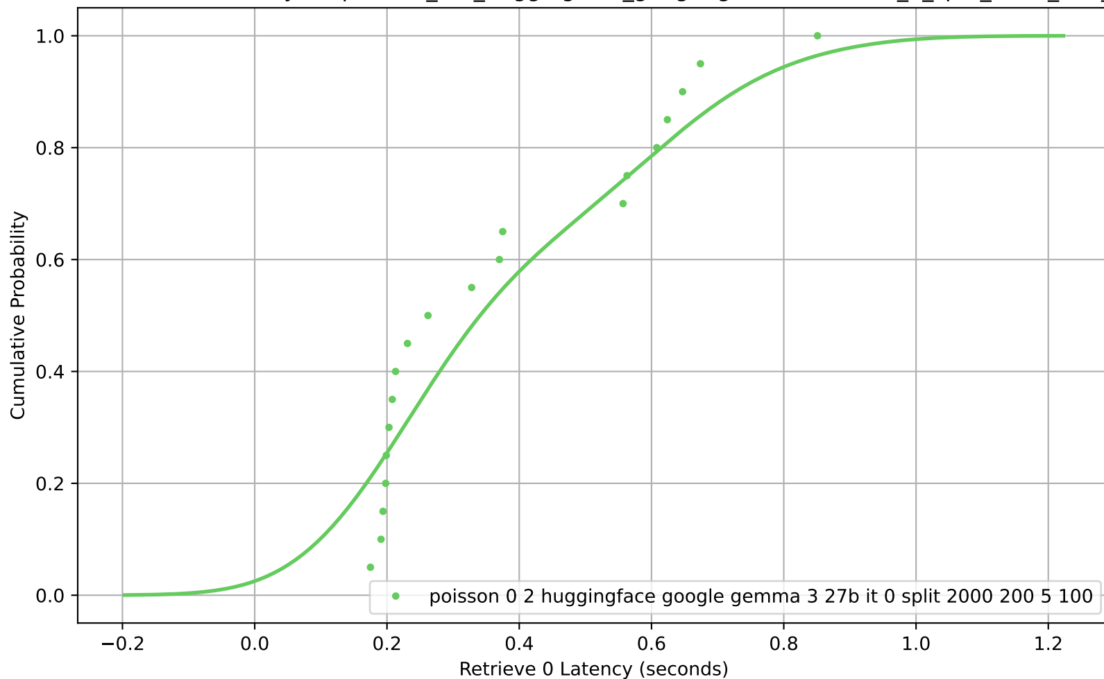
CDF of Retrieve 0 Latency for poisson_0-2_huggingface_google-gemma-3-27b-it_0_split_2000_200_5_100
