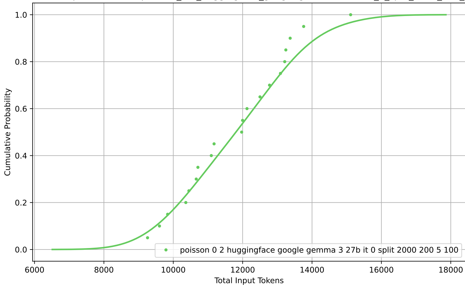
CDF of Total Input Tokens for poisson_0-2_huggingface_google-gemma-3-27b-it_0_split_2000_200_5_100
