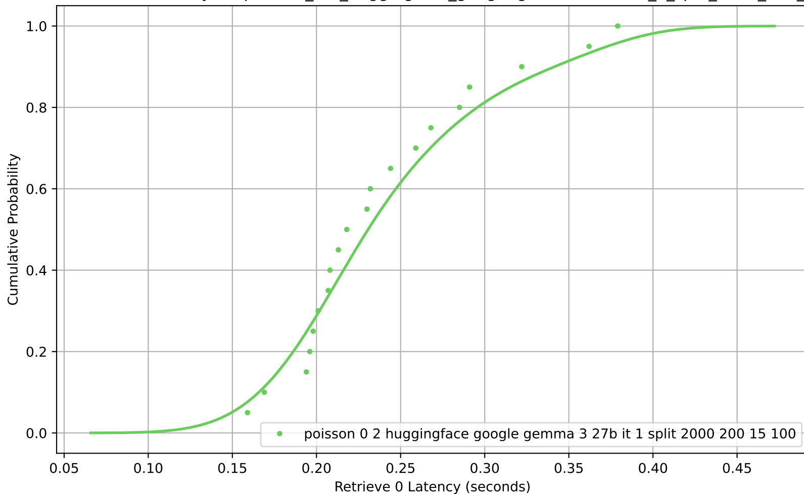
CDF of Retrieve 0 Latency for poisson_0-2_huggingface_google-gemma-3-27b-it_1_split_2000_200_15_100
