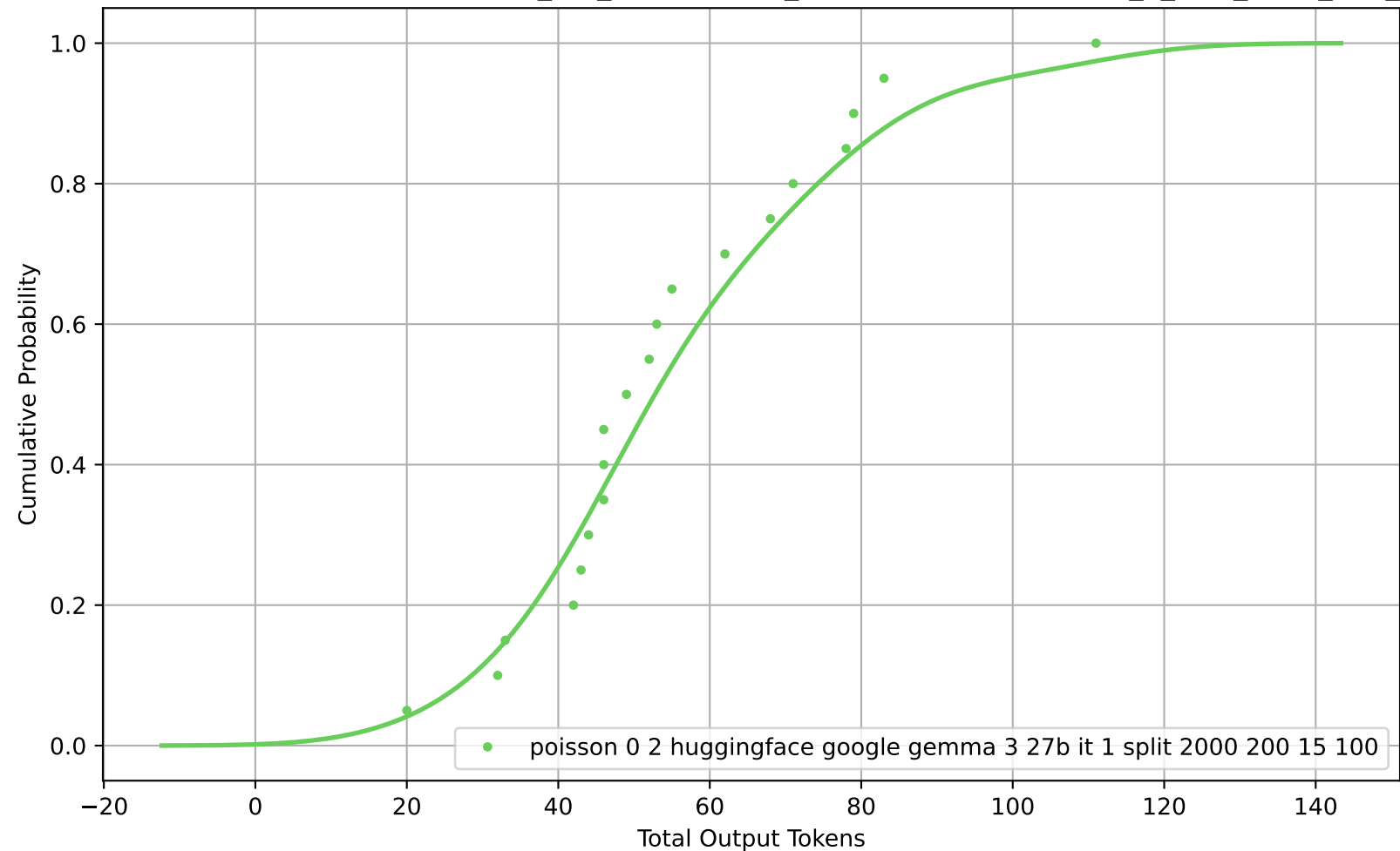
CDF of Total Output Tokens for poisson_0-2_huggingface_google-gemma-3-27b-it_1_split_2000_200_15_100
