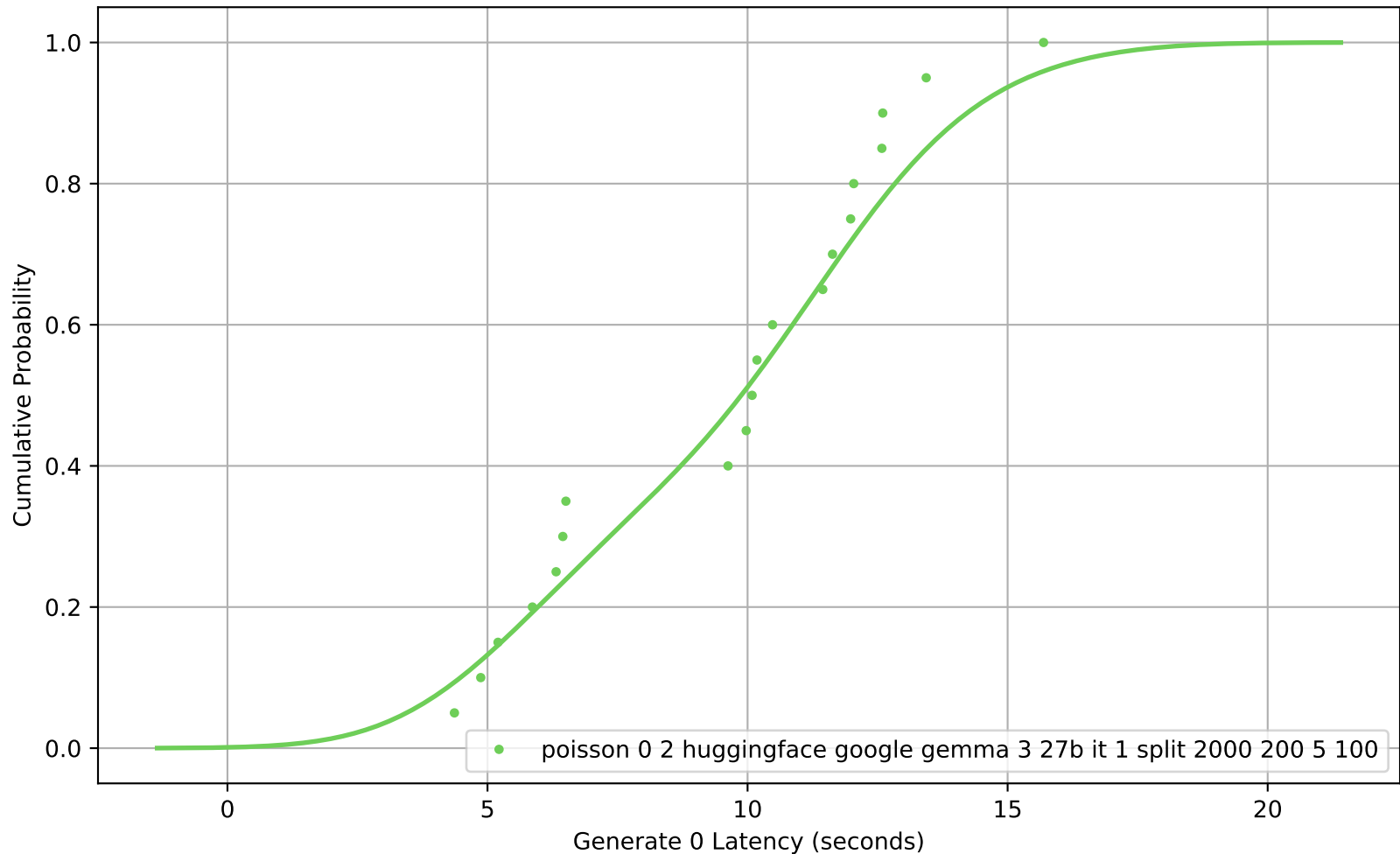
CDF of Generate 0 Latency for poisson_0-2_huggingface_google-gemma-3-27b-it_1_split_2000_200_5_100
