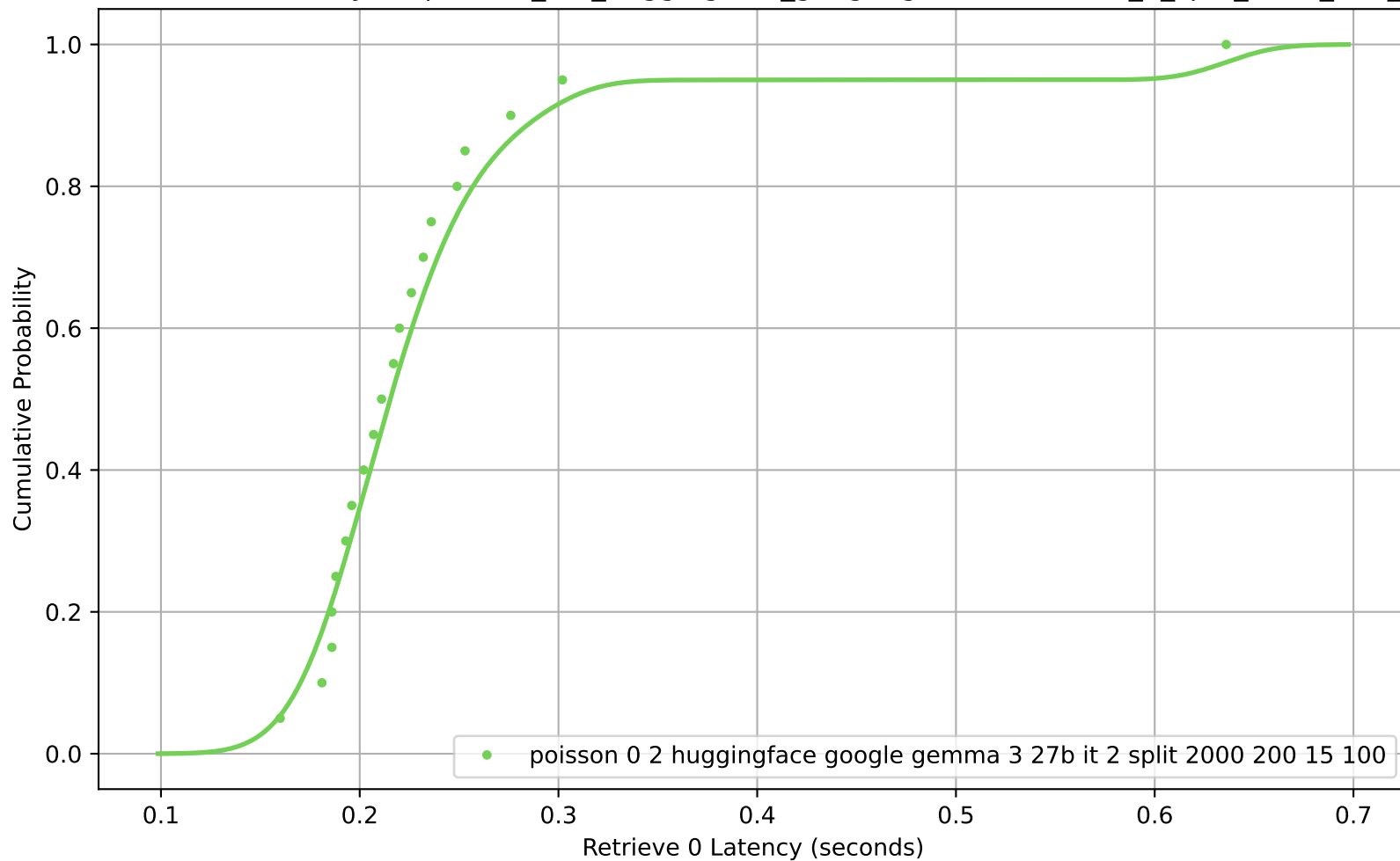
CDF of Retrieve 0 Latency for poisson_0-2_huggingface_google-gemma-3-27b-it_2_split_2000_200_15_100
