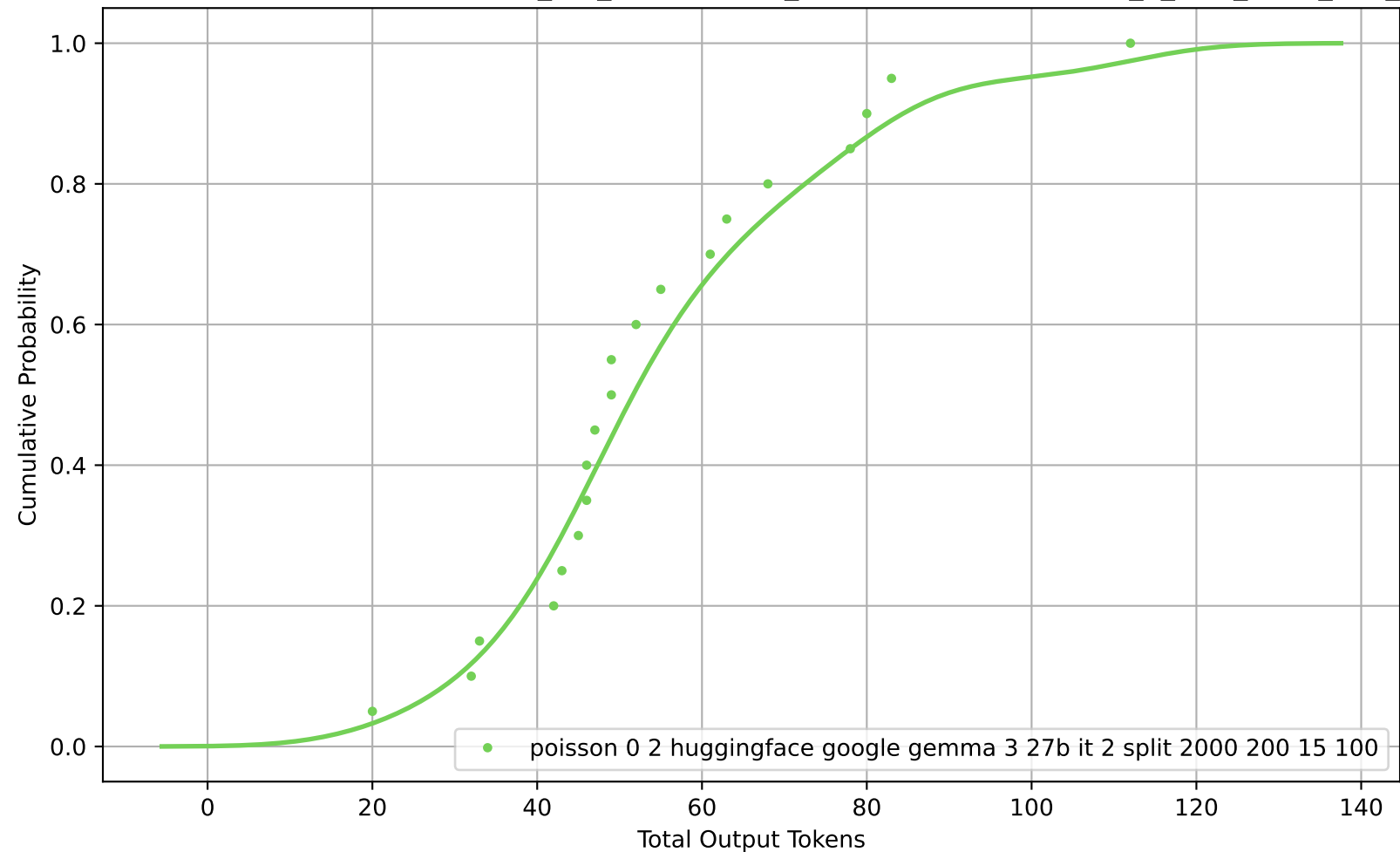
CDF of Total Output Tokens for poisson_0-2_huggingface_google-gemma-3-27b-it_2_split_2000_200_15_100
