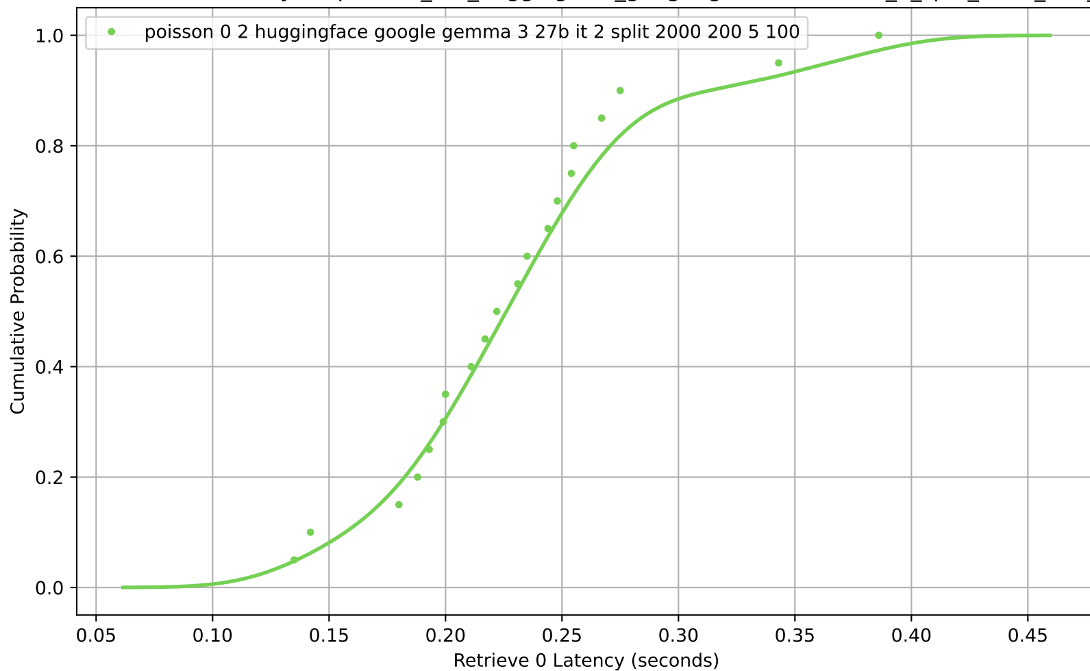
CDF of Retrieve 0 Latency for poisson_0-2_huggingface_google-gemma-3-27b-it_2_split_2000_200_5_100
